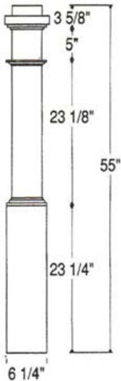
4091 Plain 4 3/4" Top Square 6 1/4" Bottom Square
