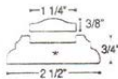
6045 Shoe Rail with Fillet
