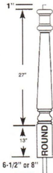
4050 3"x 41" Volute Newel Round Base with Adjustable Dowel
