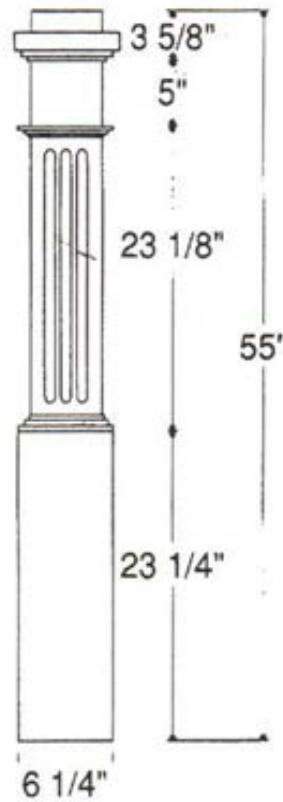
4092 Flute 4 3/4" Top Square 6 1/4" Bottom Square
