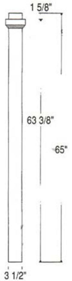
4075 Landing 3 1/2" Square
