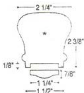
6010 P Rail with Fillet
