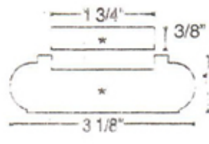
6006 Shoe Rail with Fillet
