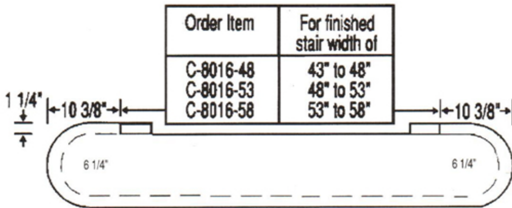
8016 Adjustable Double End Bullnose
